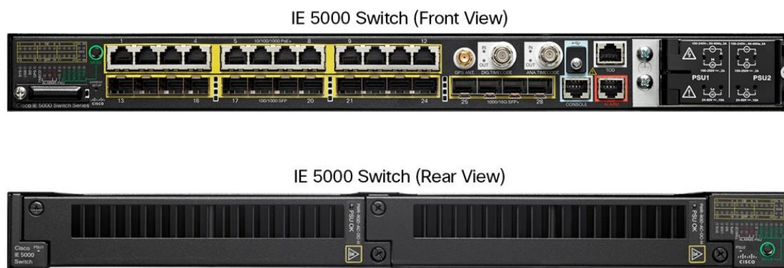
Figure 1. IE 5000 switch
