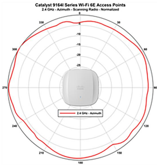
Catalyst 9164 2.4-GHz scanning radio
