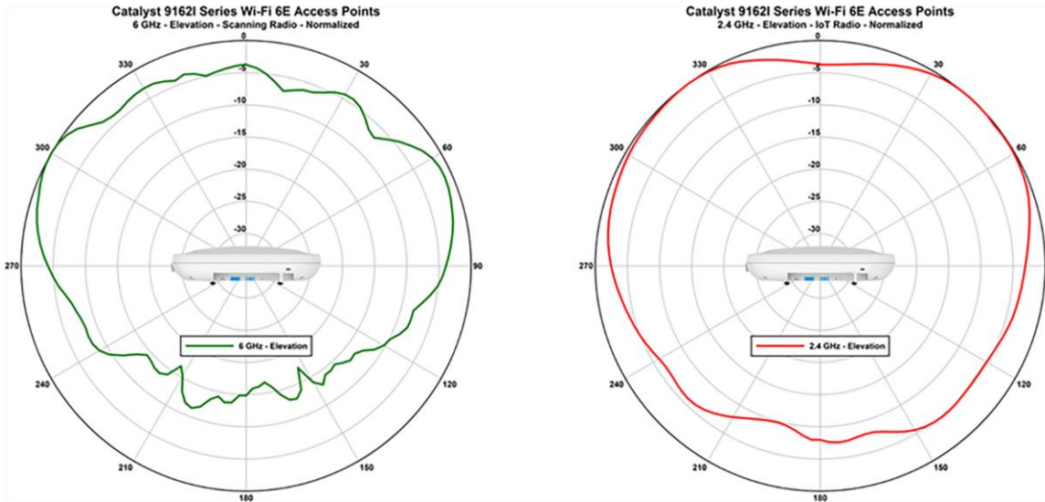
Figure 7. Antenna patterns for Catalyst 9162I 6-GHz scanning radio and 2.4-GHz IoT radio
