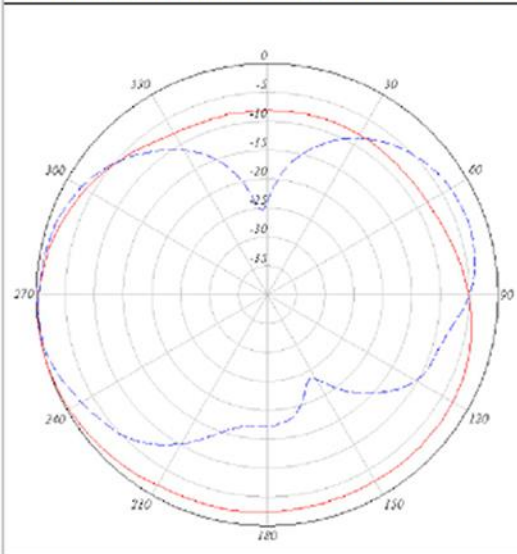
2.4-GHz Antenna 1 Azimuth and Elevation Plane Patterns
