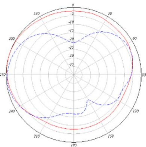
2.4-GHz Antenna 4 Azimuth and Elevation Plane Patterns
