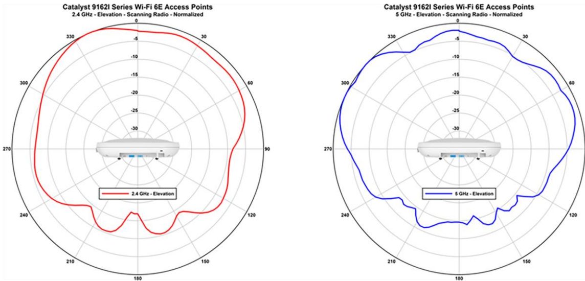
Figure 6. Antenna patterns for Catalyst 9162I 2.4-GHz and 5-GHz scanning radii
