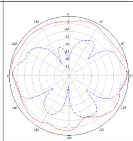
5-GHz Antenna 3 Azimuth and Elevation Plane Patterns
