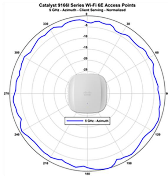
Catalyst 9166 5-GHz client serving radio
