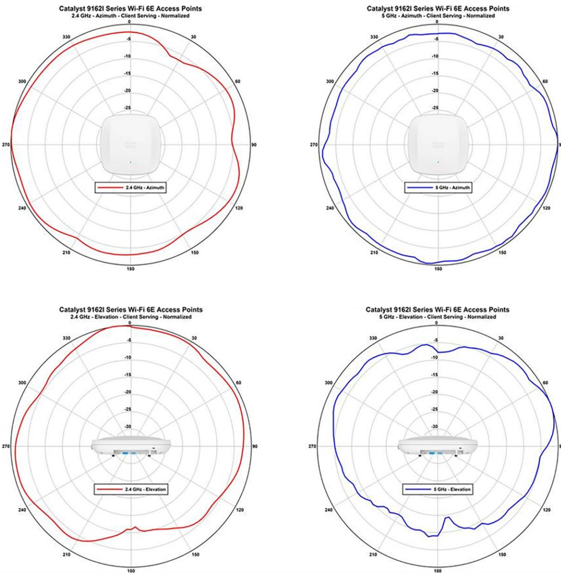
Figure 4. Antenna patterns for Catalyst 9162I 2.4-GHz and 5-GHz client serving radios
