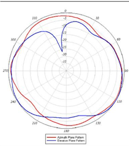
2.4-GHz Element 2 Azimuth and Elevation Plane Patterns
