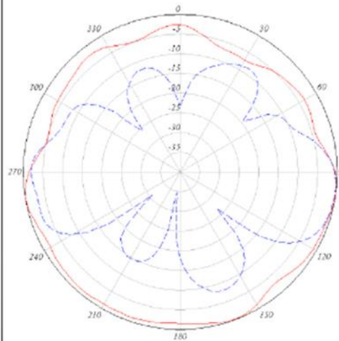
5-GHz Antenna 2 Azimuth and Elevation Plane Patterns
