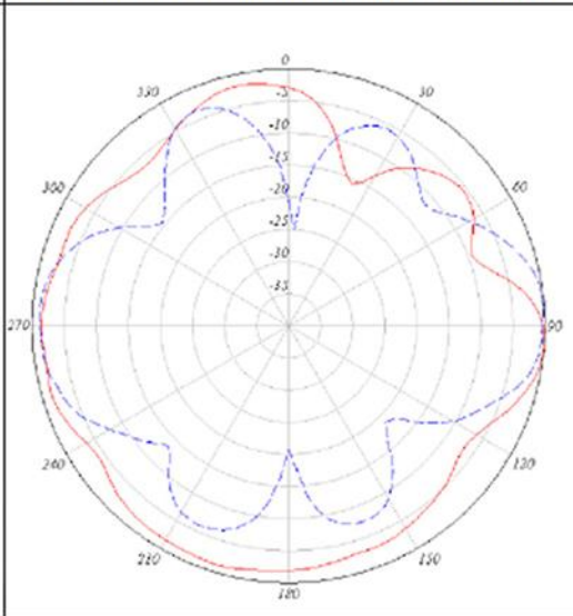
5-GHz Antenna 1 Azimuth and Elevation Plane Patterns
