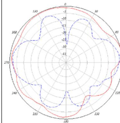
5-GHz Antenna 4 Azimuth and Elevation Plane Patterns
