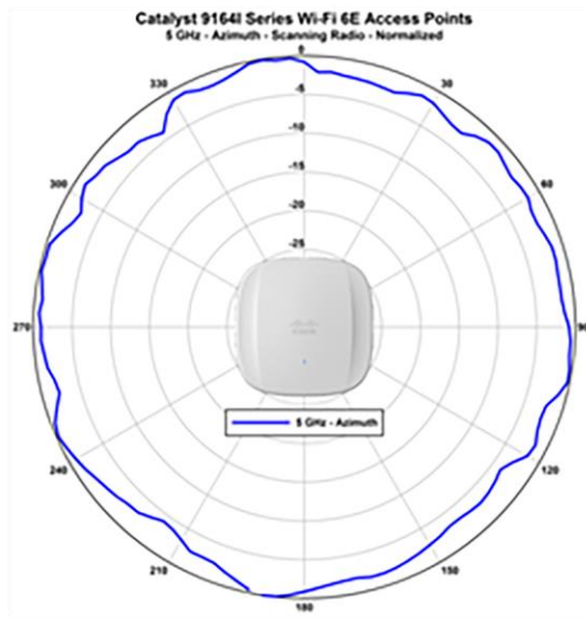
Catalyst 9164 5-GHz scanning radio
