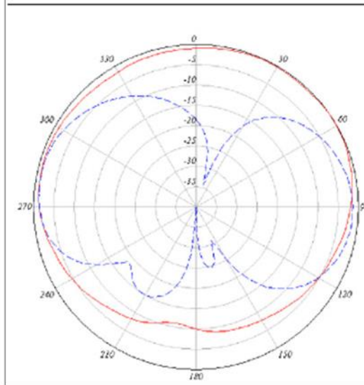
2.4-GHz Antenna 3 Azimuth and Elevation Plane Patterns
